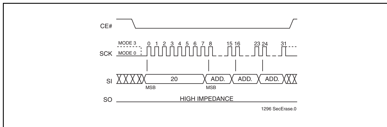
FIGURE 11: SECTOR-ERASE SEQUENCE
